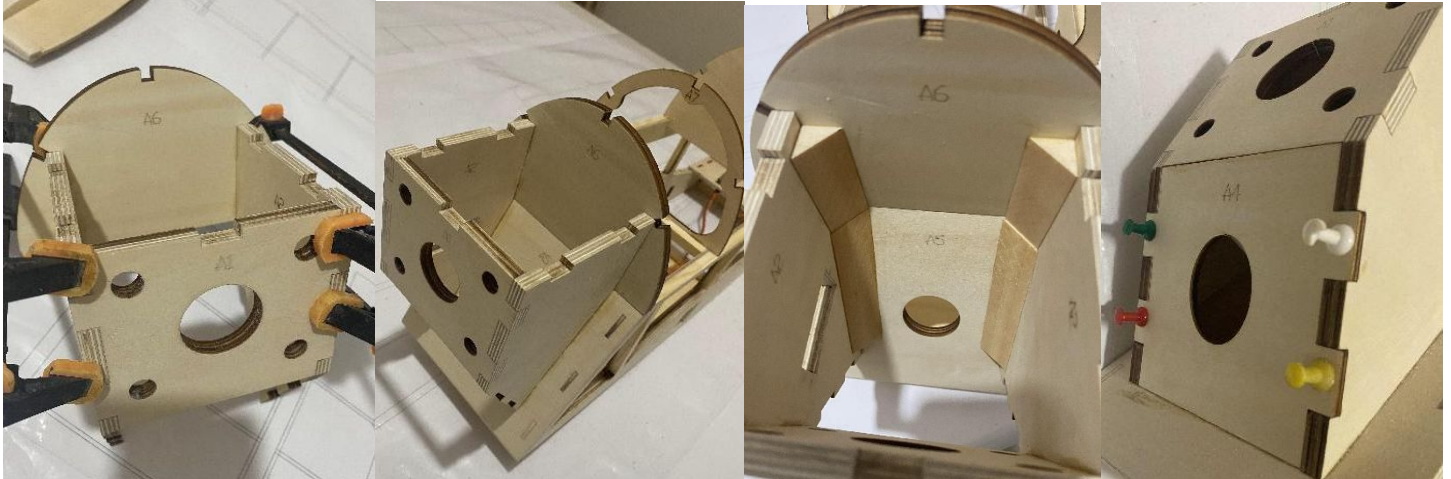
10) Install the fuselage bulkhead.
