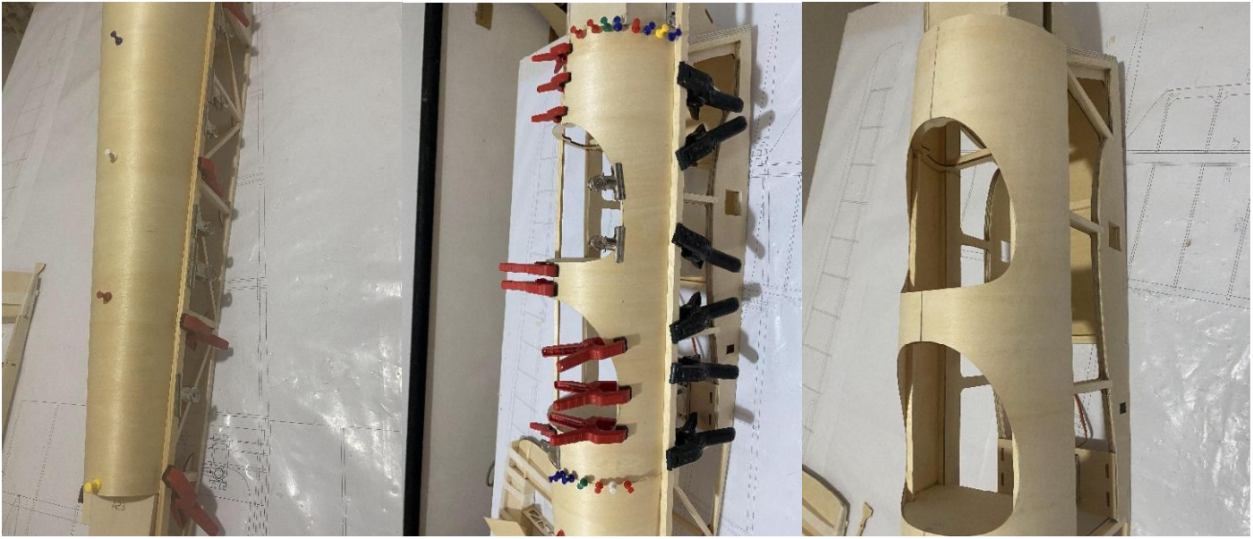
12) Glue pull-pull rods fixing seat.
