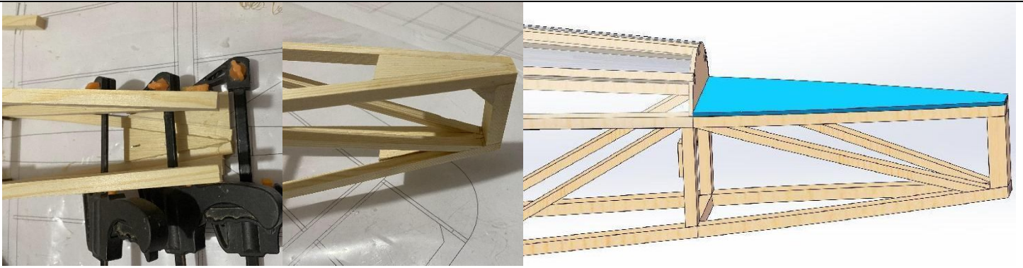
9) Glue the engine mount and use triangular wood strips for internal reinforcement.
