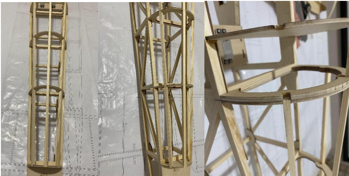
10) Install the fuselage bulkhead.
