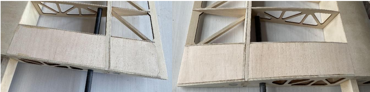
8) Fill the wing ribs with balsa strips and sand them flat.
